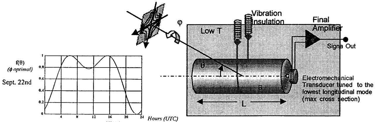
Fig. 1 Scheme of a cryogenic bar detector. The insert show the dependence on day Sept. 22 nd of the antenna pattern f(\theta, \varphi) for optimal \varphi in searching for sources at the Galactic Center.
