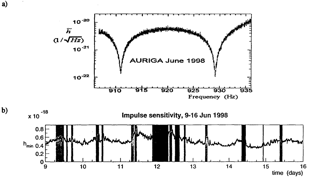
Fig. 2 a) Square root of the spectral density of noise at input (S_{hh})^{1/2} versus frequency, expressed as equivalent metric perturbation, of AURIGA (one hour average). b) The impulsive sensitivity h_{min} of Auriga over one week; the dark regions indicate interruption due to cryogenic maintenance (refill 1 Kpot of the \text{He}^3\text{-He}^4 refrigerator, refill of the main bath, etc).
