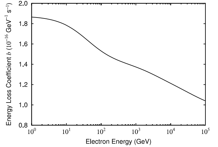
FIG. 1.—Energy-loss coefficient of cosmic-ray electrons in the Galaxy with energy. The magnetic field is assumed to be B_{\perp} = 5 \mu\text{G} .
