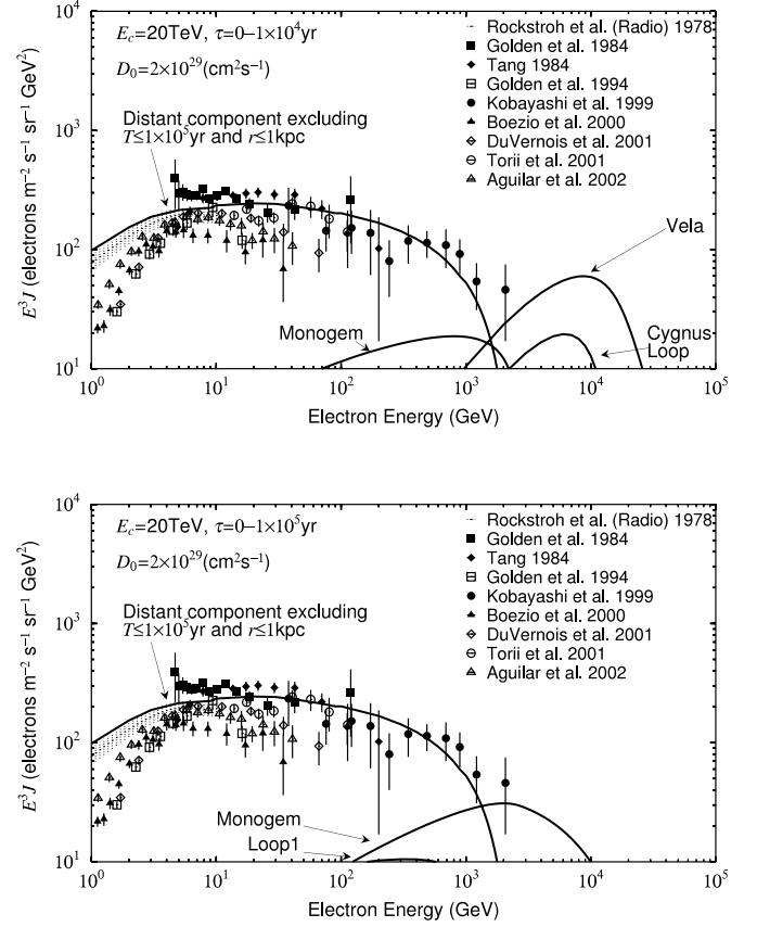
FIG. 6.—Calculated energy spectra with D_0 = 2 \times 10^{29} \text{ cm}^2 \text{ s}^{-1} and a cutoff of E_c = 20 \text{ TeV} for the continuous release of \tau = (0-1) \times 10^4 and (0-1) \times 10^5 \text{ yr} , respectively.
