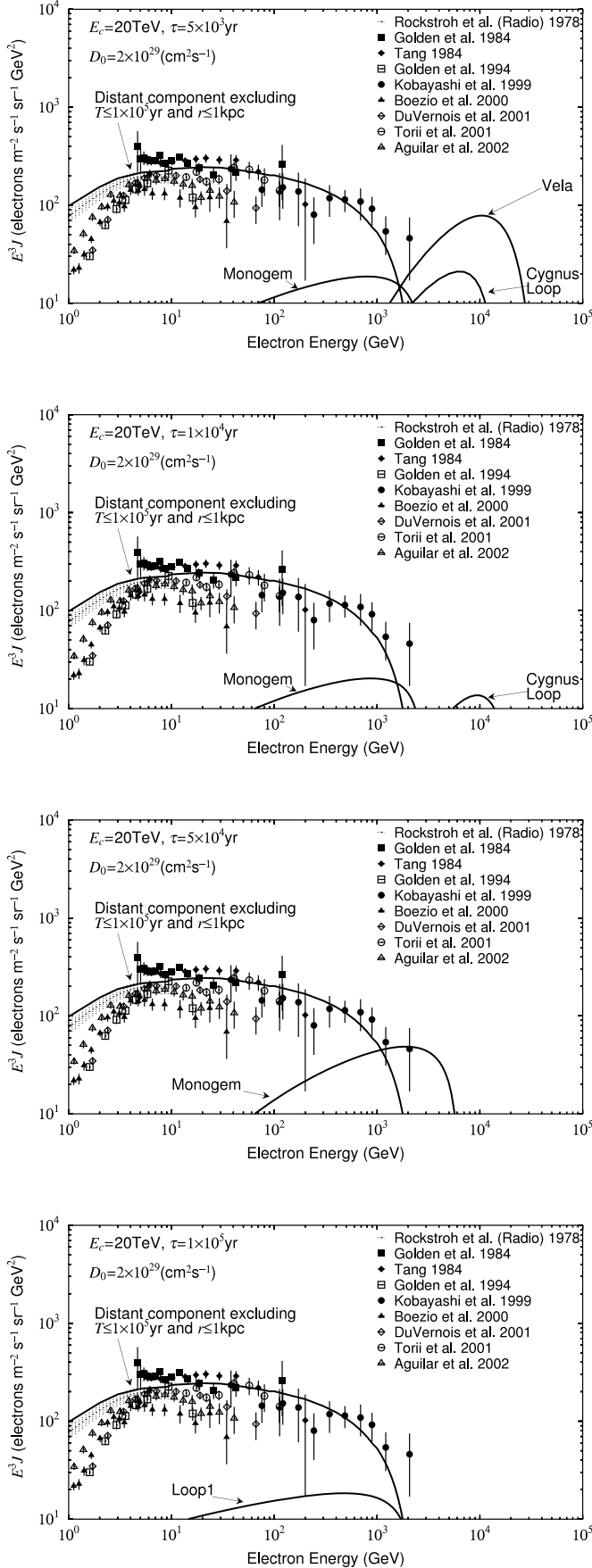
FIG. 5.—Calculated energy spectra with D_0 = 2 \times 10^{29} \text{ cm}^2 \text{ s}^{-1} and a cutoff of E_c = 20 \text{ TeV} for the burstlike release at \tau = 5 \times 10^3, 1 \times 10^4, 5 \times 10^4 , and 1 \times 10^5 \text{ yr} , respectively.
