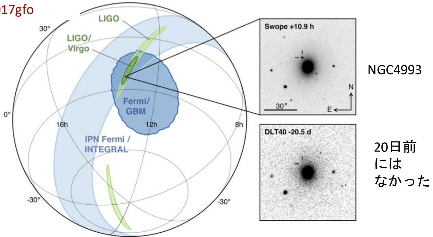
Figure 1. Localization of the gravitational-wave, gamma-ray, and optical signals. The left panel shows an orthographic projection of the 90% credible regions from LIGO (190 deg 2 ; light green), the initial LIGO-Virgo localization (31 deg 2 ; dark green), IPN triangulation from the time delay between Fermi and INTEGRAL (light blue), and Fermi -GBM (dark blue). The inset shows the location of the apparent host galaxy NGC 4993 in the Swope optical discovery image at 10.9 hr after the merger (top right) and the DLT40 pre-discovery image from 20.5 days prior to merger (bottom right). The reticle marks the position of the transient in both images.
