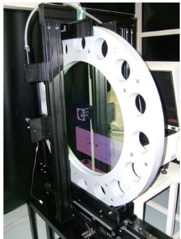
図6 開発中のすばる HSC 用狭帯域フィルター (Materion [旧 Barr Associates] 社と協力)。 Subaru/HSC narrow band filter under development (collaboration with Barr Associates Inc.)
