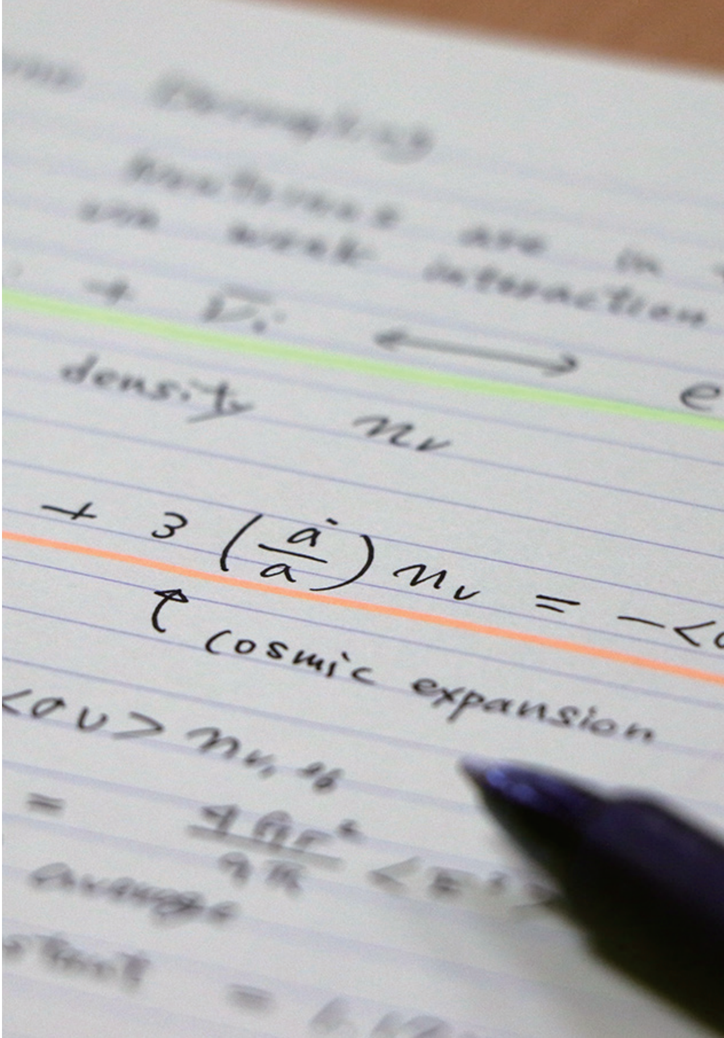
Theory
