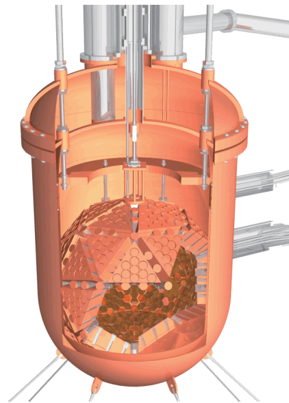
Fig. 2 The schematic view of the detector and the water tank
