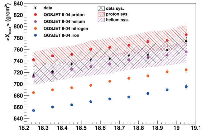
図4 TAで測定した超高エネルギー宇宙線の平均Xmaxとエネルギーの関係 (★)。赤、紫、橙、青色の丸印がそれぞれ陽子、ヘリウム、窒素、鉄モデル。 The average Xmax vs. energy of TA ultra-high-energy cosmic-ray events (★). The red, purple, orange and blue circles denote proton, helium, nitrogen and iron models, respectively.
