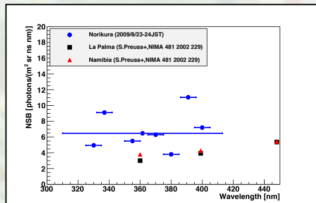
Fig. 5. Spectrum of night sky background measured at Mt. Norikura compared with those at La Palma and Namibia.
