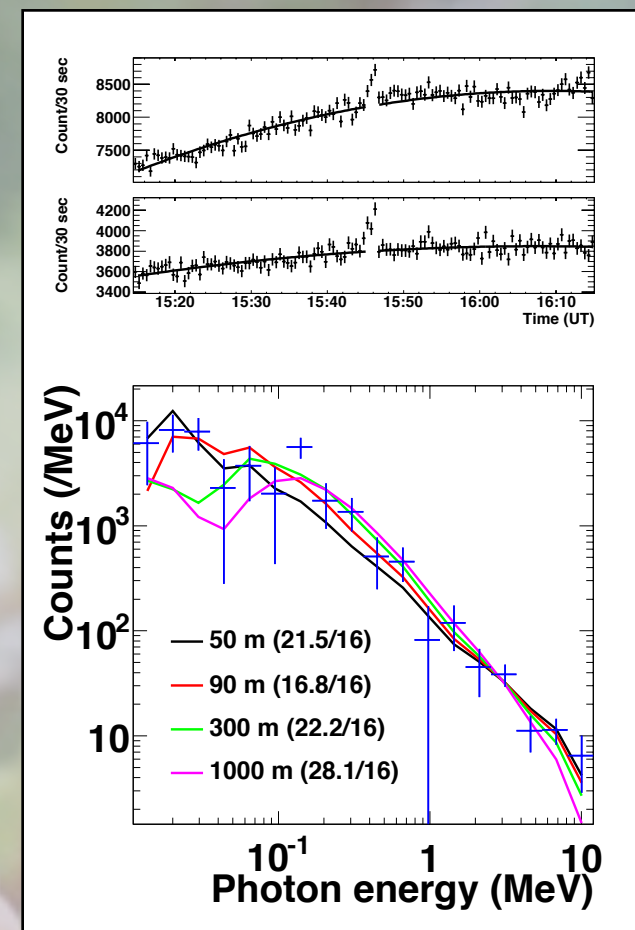
Fig. 4. (Top) Count rates per 30 sec observed by the >10 keV NaI scintillator and (Middle) by the > 100 keV plastic one. (Bottom) The photon spectrum observed by the NaI scintillator.
