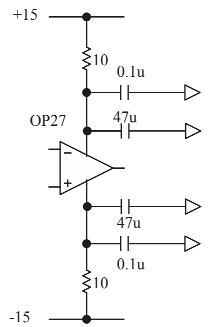
Power Supply for IC
