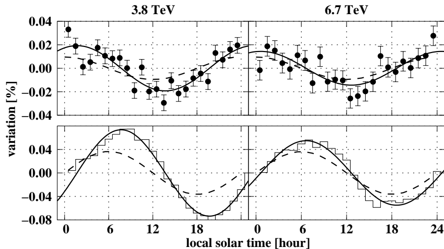
Fig. 2. Observed solar daily variations divided into energy regions compared with the expected anisotropy due to the Compton-Getting effect (the broken lines). The plot in the upper panel is the differential form of the solar daily variations, and histogram in the lower panel is physical daily variations. Solid curves are the two-parameter \chi^2 -fitted sine curves.
