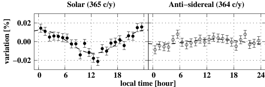
Fig. 1. The differential form of average daily variations in the local solar (left) and anti-sidereal (right) time frames, based on all the data. Broken lines show the \chi^2 -fitted sine curves which have 0.012 \pm 0.0013\% and 0.0027 \pm 0.0013\% amplitude respectively.
