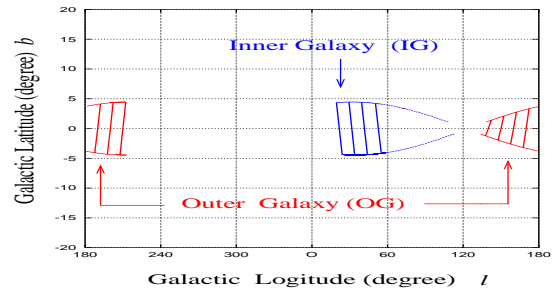
Fig. 3. IG and OG areas in the galactic coordinates corresponding to the shaded belts in figures 1 and 2.
