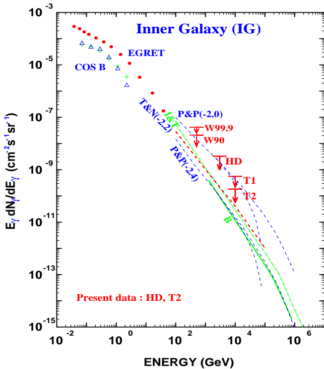
Fig. 6. Diffuse gamma rays from IG (inner galaxy). Present data are labeled by T2 and HD, and also T1 is the Tibet I data previously analyzed. Theoretical curves are labeled by initials of the first author or first and second authors names.
