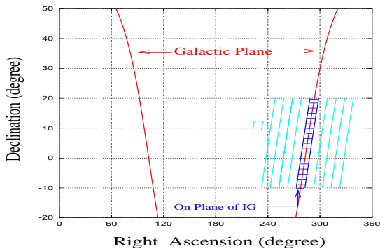
Fig. 1. 10^\circ width belts in right ascension along the galactic plane for IG near the galactic center.
