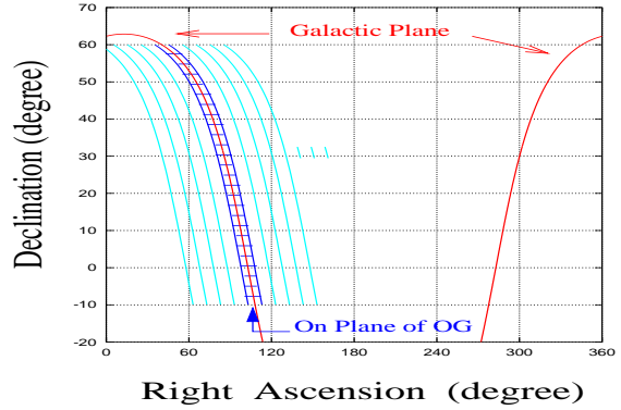
Fig. 2. 10^\circ width belts in right ascension along the galactic plane for OG around the anti-galactic center
