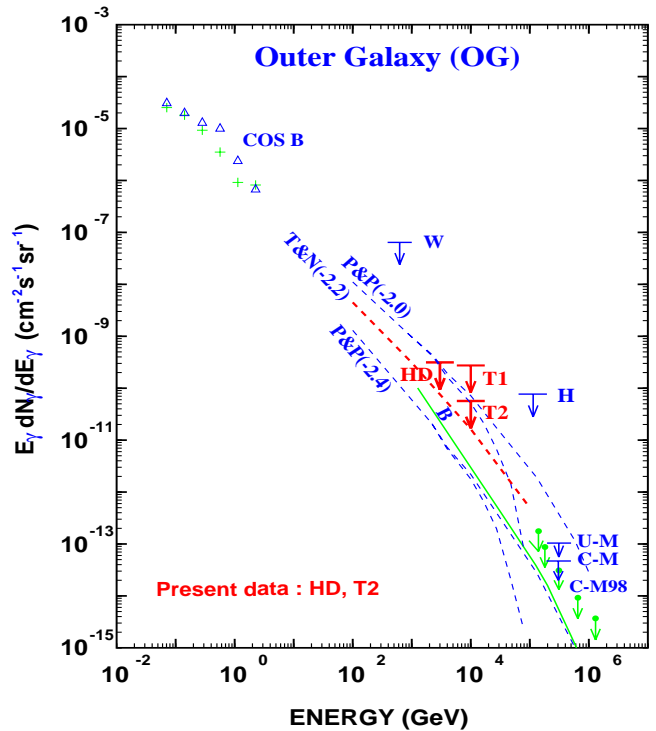
Fig. 7. Diffuse gamma rays from OG (outer galaxy). The marks and labels are same as Fig. 6. Marks W , H , U-M , C-M and C-M98 are described in the text. Present data are plotted assuming \gamma -ray spectral index 2.4 in these figures.
