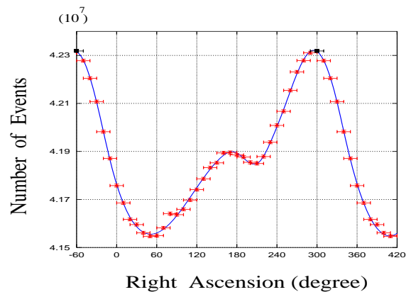
Fig. 4. Distribution of number of events in 36 curved belts for IG in the Tibet II data.
