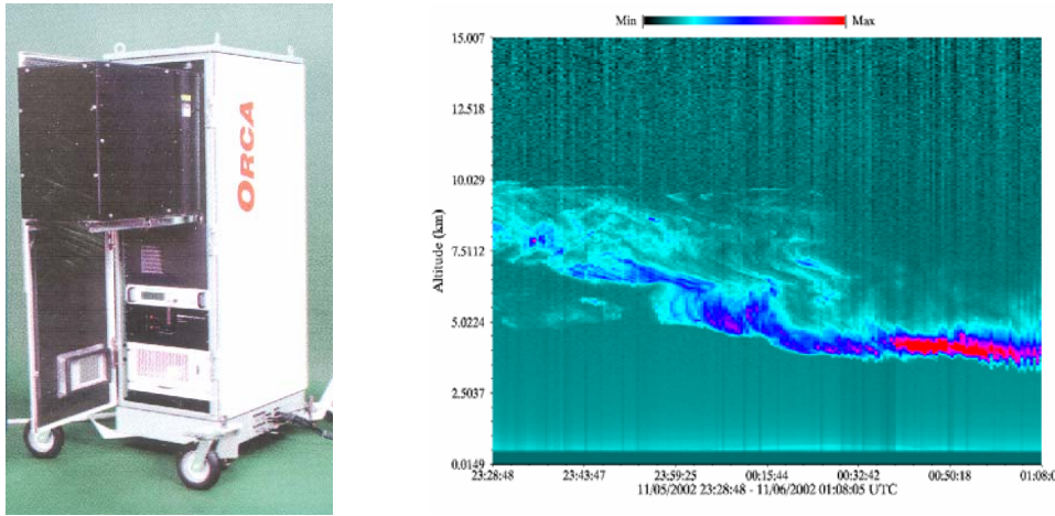
Figure 1. Left: Photo of the AROL-2 lidar system at the Space Dynamics Laboratory, Logan, Utah. Right: Altitude-time plot of lidar backscatter from the USU/SDL AROL-2 lidar, showing the development of high cirrus haze into low clouds over a 1.5-hour period near sunset (4:30-6:00 PM local) in Logan, Utah.
