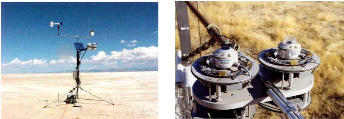
Figure 3. Left: Ventilated radiation station at Dugway, Utah. Right: Pyrgeometer (left of support) and pyranometer (right of support) for measuring incoming longwave and shortwave radiation, respectively.
