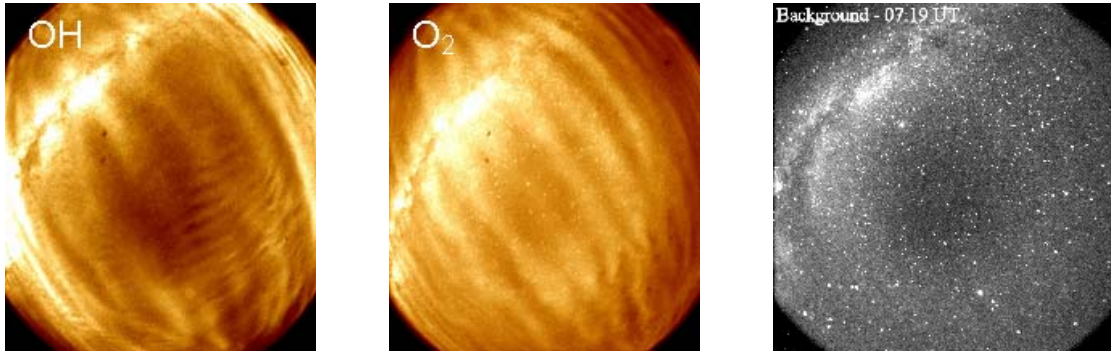
Figure 2. Left and middle: Gravity waves at the mesopause imaged with airglow emissions at two different wavelengths. Right: All-sky CCD camera background image displaying star field and diffuse atmospheric scattering of starlight.
