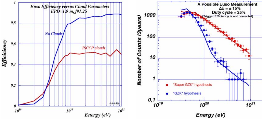
Figure 1 , Left: The detection efficiency for UHECRs by EUSO. The threshold energy is estimated at about 5 \times 10^{19} eV. Right: Expected observations of the energy distribution of events in the GZK hypothesis and in the Super-GZK hypothesis.
