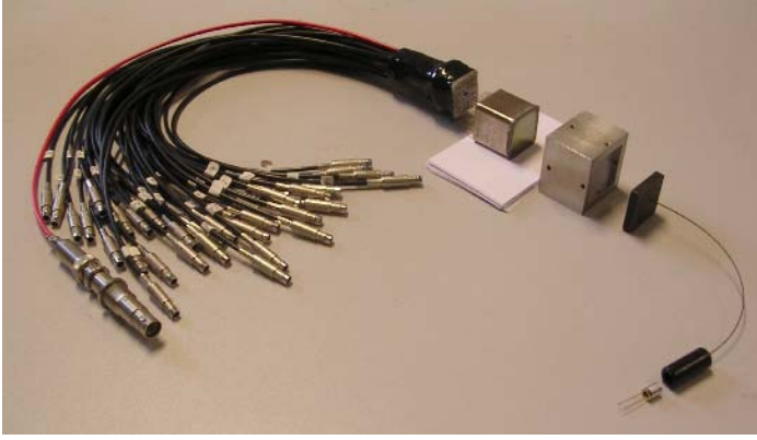
Figures 2.& 3. Exploded view of the arrangement. Down right, one can see the UV LED, followed by the coupler to the fiber. At the other extremity, the fiber goes into a 2-D comb. The intermediate aluminum piece couples exactly the fibers to the PMT which is seen next. This coupler has square holes with very thin walls, corresponding precisely to the PMT pixels. The Teflon sheet goes between the black comb and the coupler. It is pressed by the black comb against the square holes of the coupler. Finally, the Hamamatsu voltage divider is shown. The figure 3 on the right shows the photoelectrons rate in photoelectrons per second when the voltage applied to the LED is varied: red curve shows a DC voltage applied, and single pe are counted. In the blue curve the DC voltage is goes through a linear gate where it is set to 0 for 1 \mu s every 2 \mu s. The number of pe should then be exactly half of the number obtained without the gate. In the figure, the number of pe corresponding to the gate has been multiplied by two to take care of that effect. Hence, the blue curve is exactly on the red one, illustrating the system linearity.
