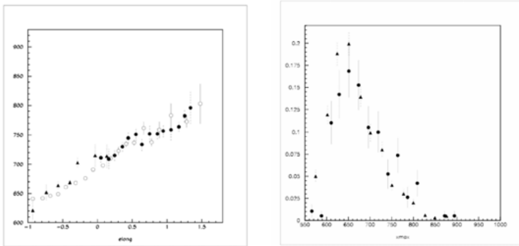
Figure 2 . Left: Elongation rate. Open circles – Stereo Fly’s Eye; Filled circles – HiRes ; Triangles – HiRes/MIA. Stereo Fly’s Eye data has been shifted by 13 gm/cm 2 . Errors are errors on the mean. Right: Xmax Distribution in 3×10 17 to 5×10 17 eV bin. Triangles: Stereo Fly’s Eye Stereo; Circles: HiRes/MIA.
