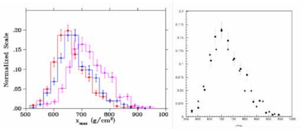
Figure 3 . Right: Xmax distribution in >10 18 eV energy bin. Triangles: Stereo Fly’s Eye; Circles: HiRes. Left: Sequence of Xmax distributions in three increasing energy bins 3-5×10 17 , 5-10×10 17 and > 10 18 eV.
