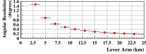
Figure 2. Expected angular uncertainties for real events as a function of the shower lever arm (see text).
