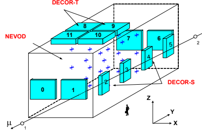
Figure 2. Experimental complex NEVOD-DECOR.
