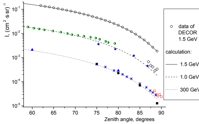
Figure 3. Dependence of absolute muon intensity on zenith angle at several threshold energies. Curves are calculation results by formula (2), values at threshold energy 1.5 GeV are multiplied by 100, at threshold energy 1 GeV are multiplied by 10. Symbols for other experiments are the same as in Fig. 1.
