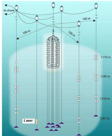
Figure 1. NT200+: the old NT200 telescope surrounded by 3 new strings at 100 m radius. The new NT200+ laser is indicated; central DAQ is located in left upper unit.
