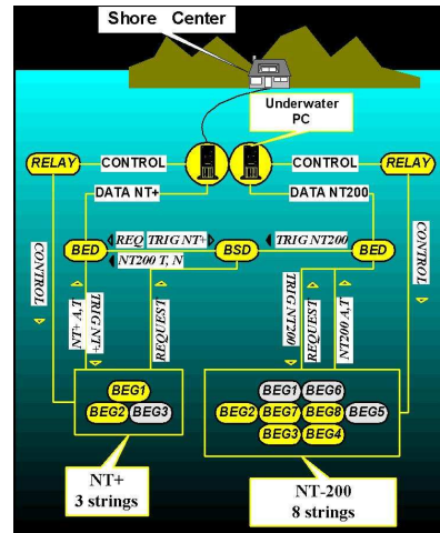
Figure 2. Sketch of data collection and slow control in NT200+: 8-string telescope NT200 and 3 new outer strings (“NT+”), controlled from two underwater PCs (see Fig.3).
