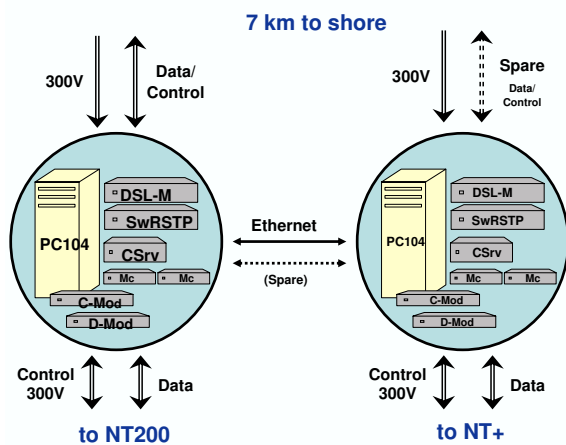
Figure 3. Sketch of the new NT200+ central DAQ/Control spheres with embedded PC104, redundant network components, and the experiment bus interfaces. See also Fig.2.
