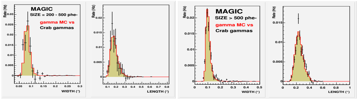
Figure 2. Distribution of the WIDTH and LENGTH parameters of shower images for Monte Carlo gammas (shaded histograms) and real Crab gammas (crosses).left: SIZE between 200 and 500 \text{phe}^- (corresponding to a gamma peak energy of 140 GeV); right: SIZE > 500 \text{phe}^- (peak energy 270 GeV).
