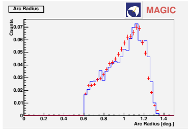
Figure 3. The distribution of the radius R_{arc} of the fitted muon rings is shown for data (red dots) and MC (blue histogram)
