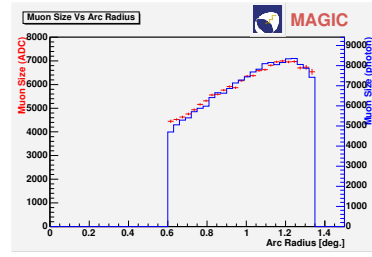
Figure 4. The dependence of SIZE_{muon} on R_{arc} is shown for data (red dots) and MC (blue histogram). After overall CE calibration good agreement is achieved.
