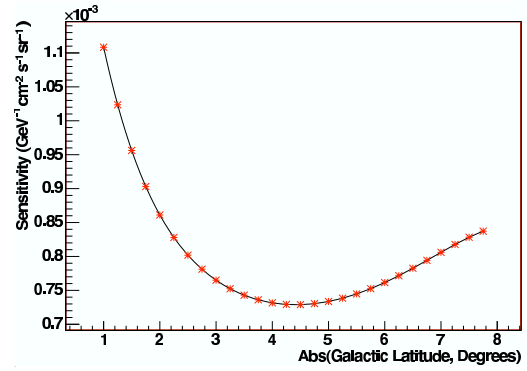
Figure 3. Sensitivity to a Gaussian source ( \sigma = 2.1^\circ ) as a function of on-source region size.
