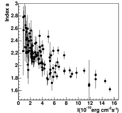
Figure 3. Correlation of RXTE-PCA spectral index “a” and integral flux over 4-15 keV.
