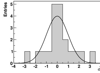
Figure 1. Distribution of the significance observed from the 20 selected AGN. The curve represents a Gaussian distribution with zero mean and a standard deviation of one.
