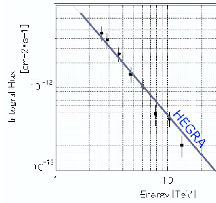
Figure 4. Integral flux of the Crab nebula.
