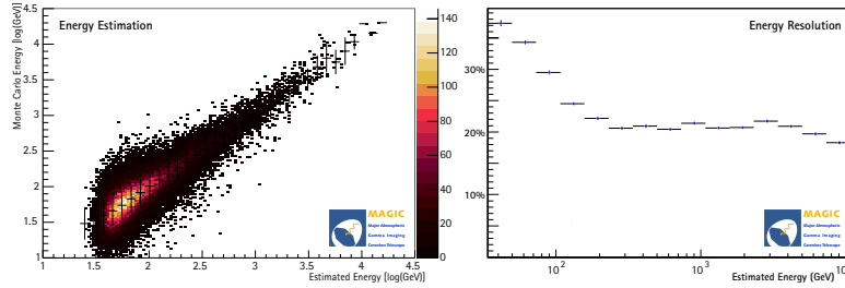
Figure 3. Left: Estimated energy vs. true energy, for Monte Carlo events. Right: Energy resolution as a function of (estimated) energy.
