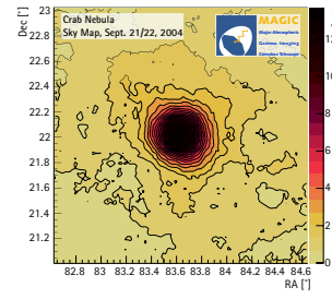
Figure 2. Disp-Sky map for the Crab nebula.
