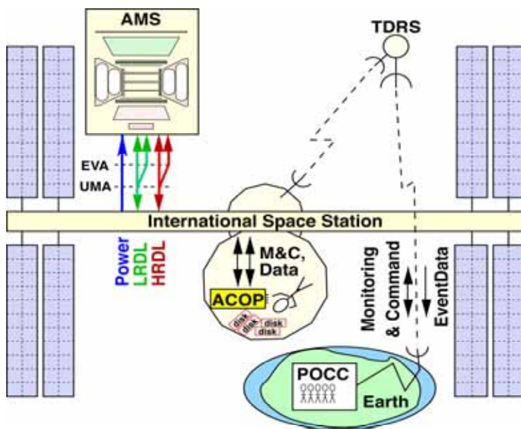
Figure 1. AMS electrical interfaces on ISS (TDRS: Tracking and Data Relay Satellite, POCC: Payload Operations and Control Center, M&C: Monitoring and Command).
