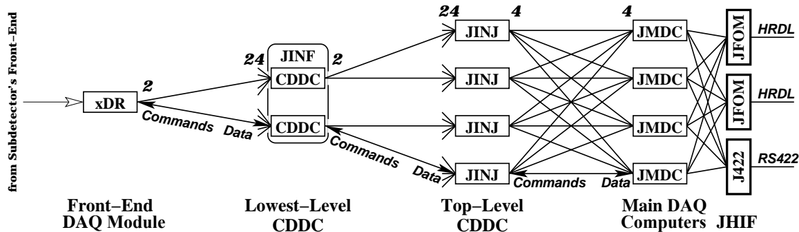
Figure 4. The DAQ tree. The number of redundant nodes at each level is shown.
