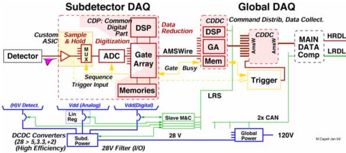
Figure 2. Unified approach to subdetector electronics for DAQ, Monitoring and Control (M&C) and power.
