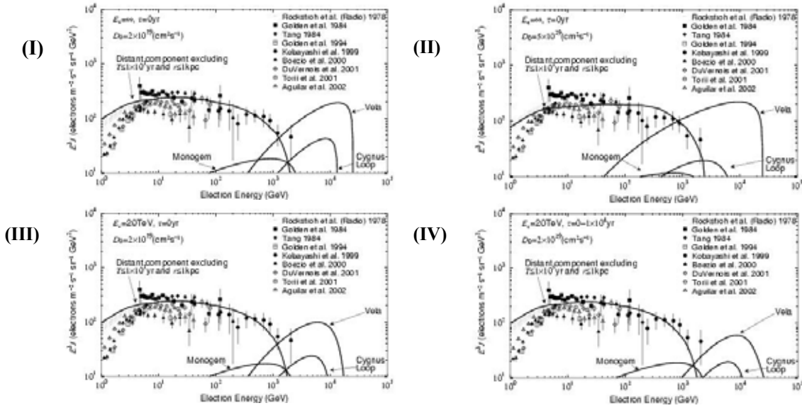
Figure 1. Expected energy spectrum of electrons from a diffusion model calculation under different assumptions, comparing with the present data. The assumptions are following: (I) no cut-off energy ( E_c = \infty ), instant acceleration time ( \Delta T = 0 yr) and the diffusion coefficient at 1 TeV of D_0 = 2 \times 10^{29} cm 2 /s. (II) D_0 = 5 \times 10^{29} cm 2 /s. (III) E_c = 20 TeV. (IV) E_c = 20 TeV and \Delta T = 10^4 yr. The parameters not shown in (II), (III) and (IV) are same with (I).
