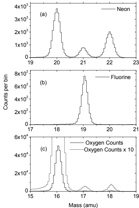
Figure 1—Mass histograms of neon, fluorine, and oxygen isotopes
