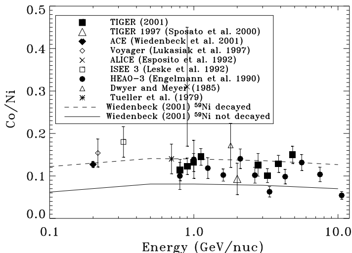
Figure 2. TIGER 2001 results for Co/Ni at the top of the atmosphere as a function of energy compared with data from previous experiments and with an interstellar propagation model [12].
