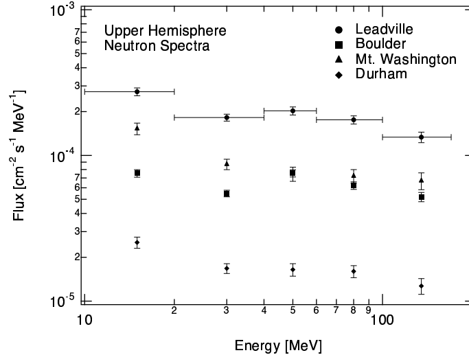
Figure 1. Upper hemisphere neutron spectrum at four sites during in 1987.
