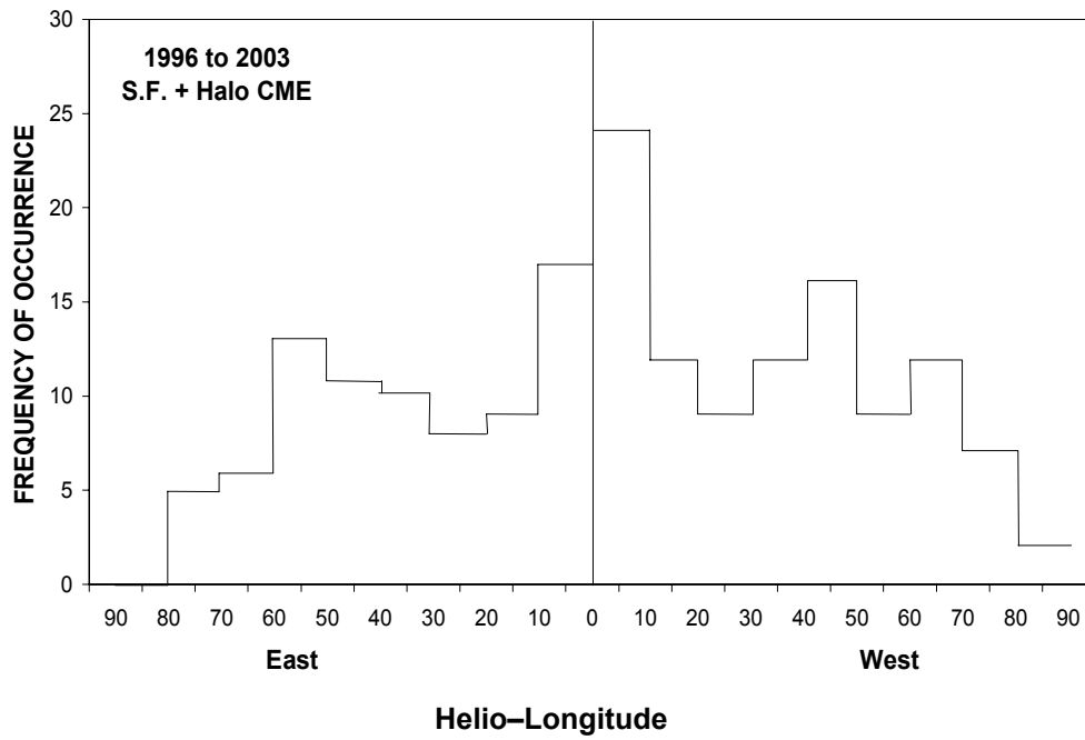
Figure 1. Shows the frequency of occurrence of solar flares with helio-longitude in interval of 10° for the period of 1996 to 2003. The group of 182 solar flares are in association with halo CMEs.
