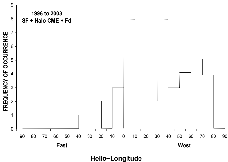
Figure 2. Shows the frequency of occurrence of solar flares with helio-longitude in interval of 10° for the period of 1996 to 2003. The group of 44 solar flares are in association with halo CMEs and Fds.
