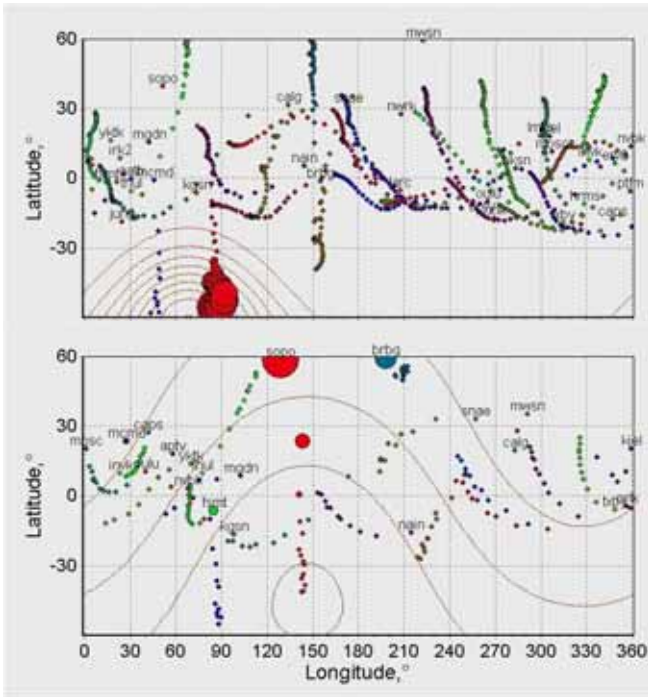
Figure 3. Asymptotic directions for particles of different energy recorded at each station at the just after the onset of GLE69 (6:50-6:55) and at 11:15-11:20 UT.
