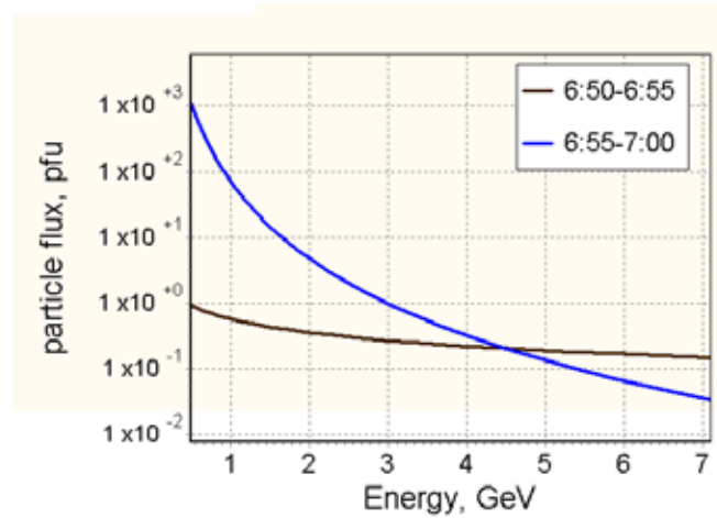
Figure 4. Spectra of the solar CR during the first and second 5-minute intervals after the onset.
