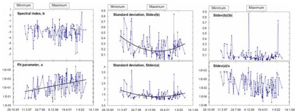
Figure 2. The evolutions of the power law fit parameters during the solar cycle 23. The approximate solar activity minimum and maximum are marked at the top of the panels.
