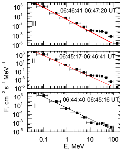
Figure 3. The energy spectra of gamma rays observed by SONG during three time intervals marked in Figure 2.
