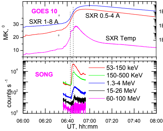
Figure 1. Upper panel: Soft X ray measurements by GOES on 20 January 20 2005. Lower panel: Excess on hard X ray and gamma channels observed by SONG on CORONAS-F.
