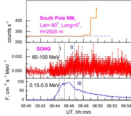
Figure 2. The temporal profile of measurements at two gamma ray channels of SONG along with the onset of GLE observed on South Pole NM.
