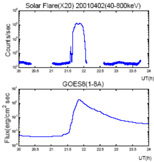
Figure4 The brightest solar flare in the 23 rd cycle. SF 010402 by SZ2/XD2 and GOES8(down)
