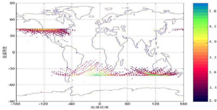
Figure6 Burst-like electron events(PPE) measured in Jan-Jun. The SAA regions were mostly excluded by switching off the HV of PMT. The flux shown on SAA regions was is from the first several days when the HV control program did not work.
