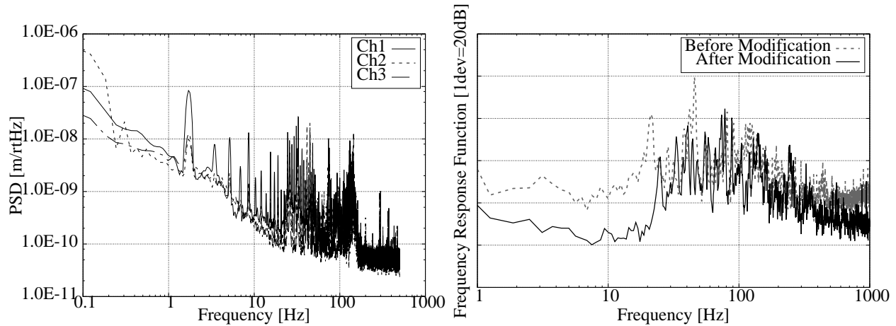
FIGURE 5. (LEFT) Measured typical power spectral density (PSDs) for the direction along the 8 K thermal conduction bar (Ch 1), horizontal perpendicular to the bar (Ch 2), and for the vertical (Ch 3). This is measured after the modification of the support structure. (RIGHT) The frequency response functions (FRFs) of the cryocooler unit obtained by the hammering test. The results before and after the modification of supporting structures are shown.
