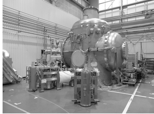
FIGURE 3. (LEFT) Pictures of the cryocooler unit testing its thermal and vibration performance. The test jig was attached to the end of thermal paths for the stand alone test. (RIGHT) Picture of the cryostat. Three of four cryocooler units are shown around the cryostat. Round-shape closing flanges at side will be connected to the beam tubes.
