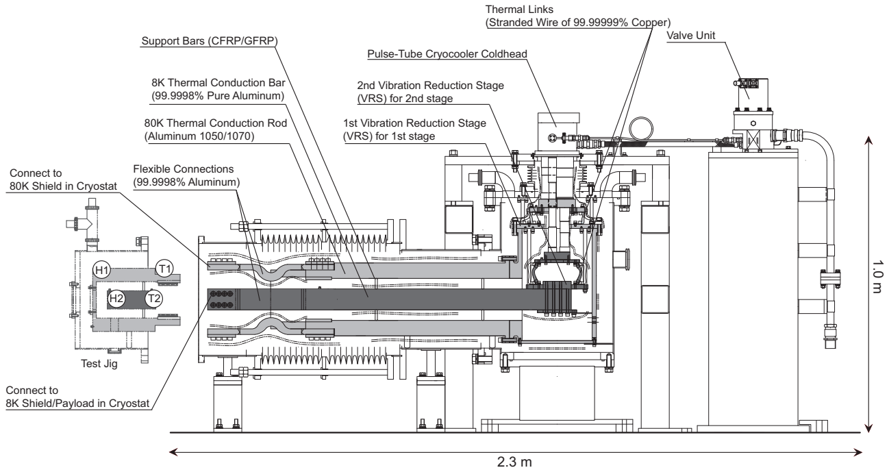
FIGURE 2. The sectional view of the very-low-vibration cryocooler unit. 8 K thermal conduction bar is colored in dark gray and the 80 K thermal conduction rod is colored in light gray. Test jig is attached to the end of the thermal paths for stand alone performance tests. T1 and T2 represent the location of temperature sensors for the test, and H1 and H2 represent that of heaters.
