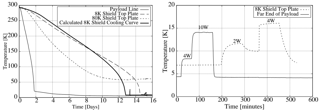
FIGURE 6. (LEFT) Typical cooling curves obtained from the cooling performance test of the cryostat No.2. (RIGHT) Typical temperature responses to the input heat load at the payload line and 8 K shield obtained from the test of the cryostat No.1.
