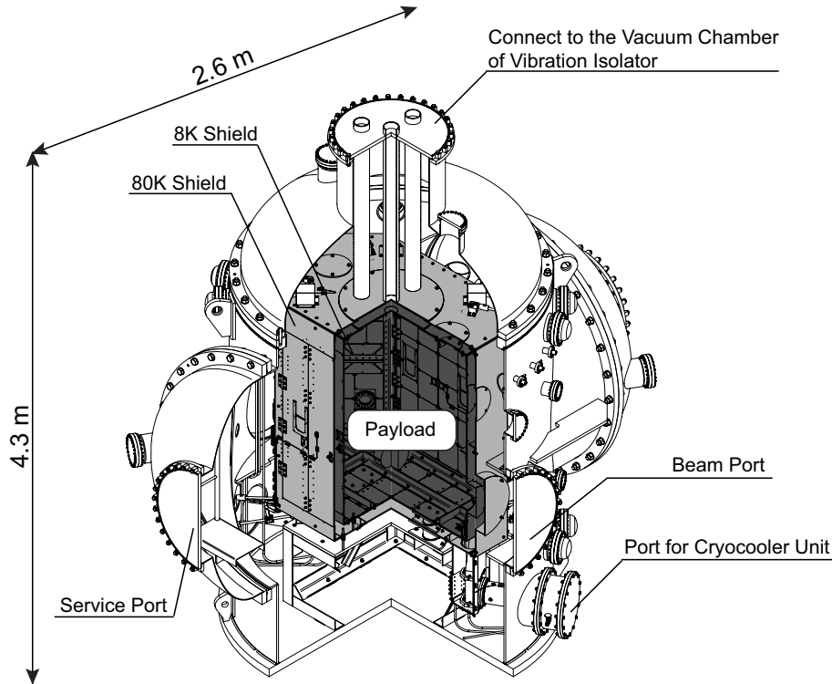
FIGURE 1. One-quarter cut section view of the cryostat. The dark-gray color is on the 8 K shield and the light-gray color is on the 80 K shield. Mirror and other components for the interferometer are not shown in this figure. MLI is also not shown here.
