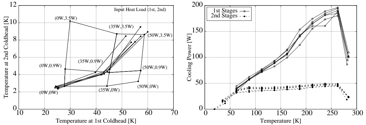
FIGURE 4. (LEFT) Measured load map of the SHI RP-082B PT cryocoolers. Seven cryocoolers out of sixteen were measured by two different heat load such as 35 W/0.9 W and 50 W/3.5 W for 1st/2nd stage respectively, and one of them was measured in detail by giving additional heat loads. (RIGHT) Measured cooling power of the cryocooler units at each temperature [6].
