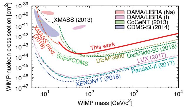
図6 WIMPs の感度曲線。様々な検出器による結果も書かれている。赤線 (This work) が今回の結果。下に行くほど感度が良いことになる。 The spin-independent WIMP-nucleon cross section limit as a function of the WIMP mass at the 90% CL for this work is the solid red line. Limits as well as allowed regions from other experimental results are also shown.
