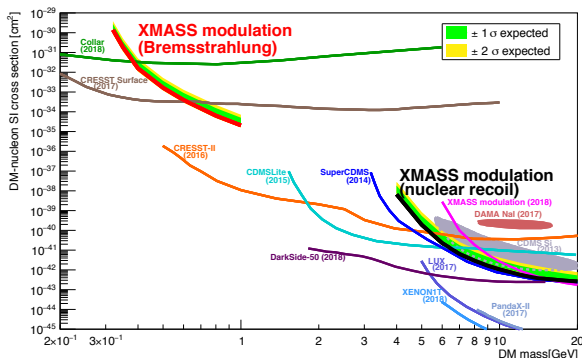
図3 赤線は bremsstrahlung 放射の効果を取り入れた 0.32-1 GeV/c 2 の質量領域での結果。黒線は弾性散乱の解析手法を用いたもの。緑と黄色の領域はそれぞれ \pm 1\sigma と \pm 2\sigma の感度領域を示している。 The red line shows the result of bremsstrahlung analysis carried out by XMASS for 0.32-1 GeV/c 2 DM mass and the black line for result of the nuclear recoil search. Several searched by other experiments are also shown for comparison. The green and yellow bands are the \pm 1\sigma and \pm 2\sigma expected sensitivity of 90% CL upper limits, respectively.
