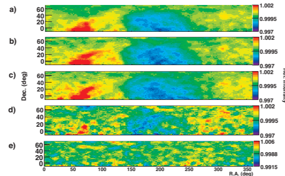
5 恒星時宇宙線異方性 (上から 4, 6.2, 12, 50, 300TeV) Cosmic ray anisotropy at sidereal time frame for 4, 6.2, 12, 50, 300TeV from above.
