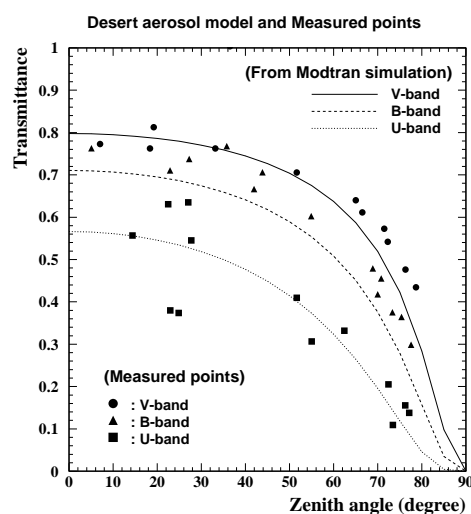
Figure 3. Comparison of measurements and simulation. Color represents each wavelength range as same in Fig 2. Points represent measurement data and lines represent the results of Modtran simulation (‘Mid-Latitude Winter’ model atmosphere with ‘desert aerosol model’).
