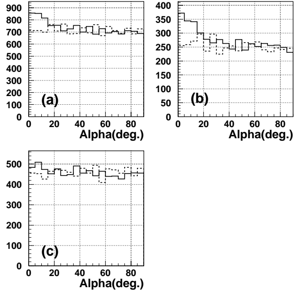
Fig. 1. (a) Plot of the event distribution as a function of the \alpha for the 1997 data. (b) is the similar plot after applying the timing selection, and (c) is also the similar plot for rejected events of (a) by this cut.
