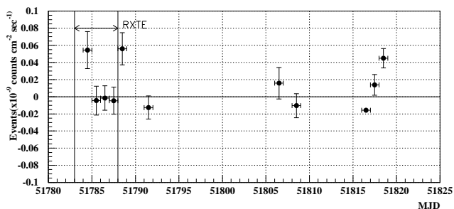
Fig. 3. The number of excess events for PKS 2155–304 night by night. Vertical error bars indicate 1\sigma statistical errors.
