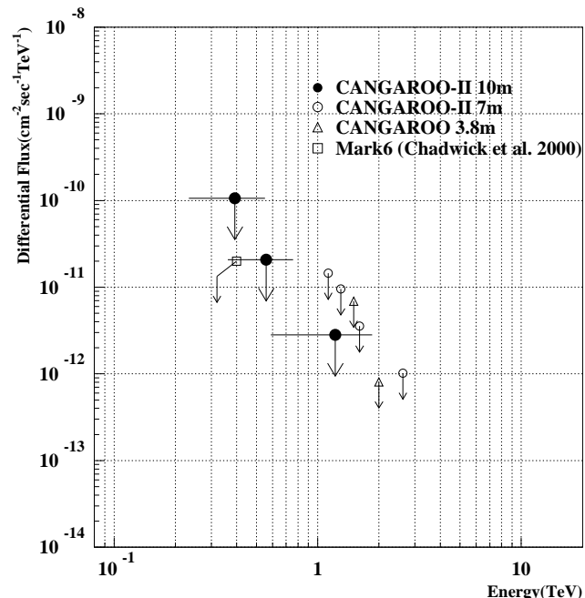
Fig. 2. Differential energy spectrum of PKS 2005–489. The 2\sigma flux upper limits from the present work are denoted by the closed circles. The open circles and open triangles show the upper limits obtained from quick-look analysis of CANGAROO-II 7m observation and from CANGAROO 3.8m observation (Roberts et al., 1998a,b), respectively. Open square indicates the upper limit reported by Chadwick et al. (2000).
