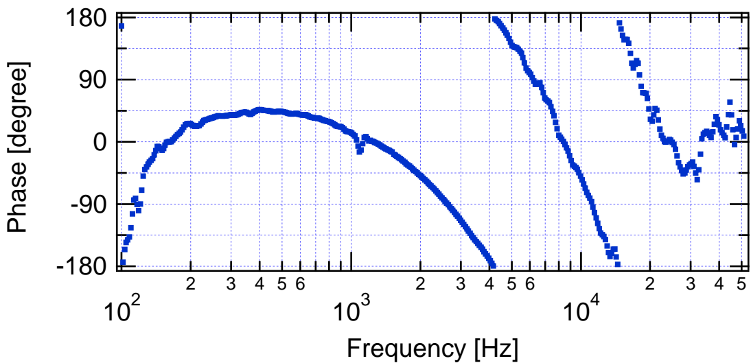
Open loop TF (suspension cavity)
